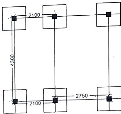
LAYOUT PLAN
