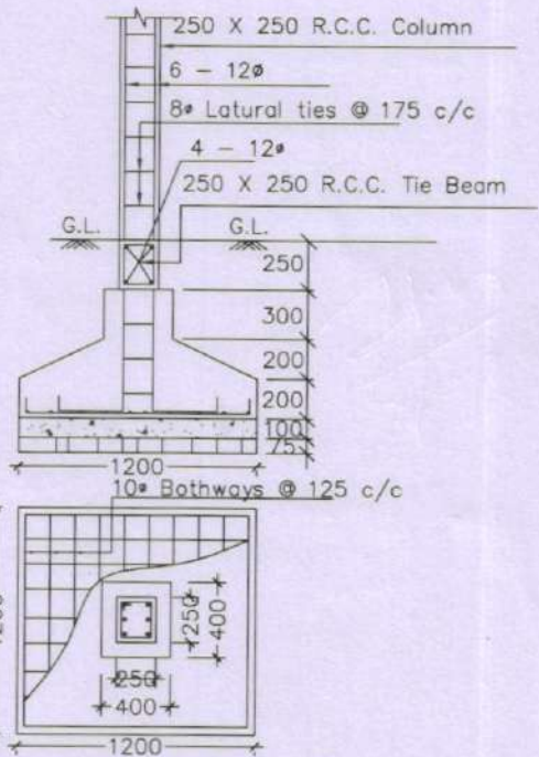
DETAILS OF R. C. C COLUMN (SCALE - 1 : 25)
