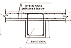
Slab Beam Details
