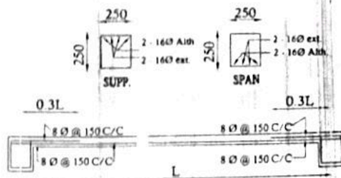
Details Of R.C.C Roof Slab & Beam
