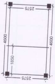
LAYOUT PLAN
