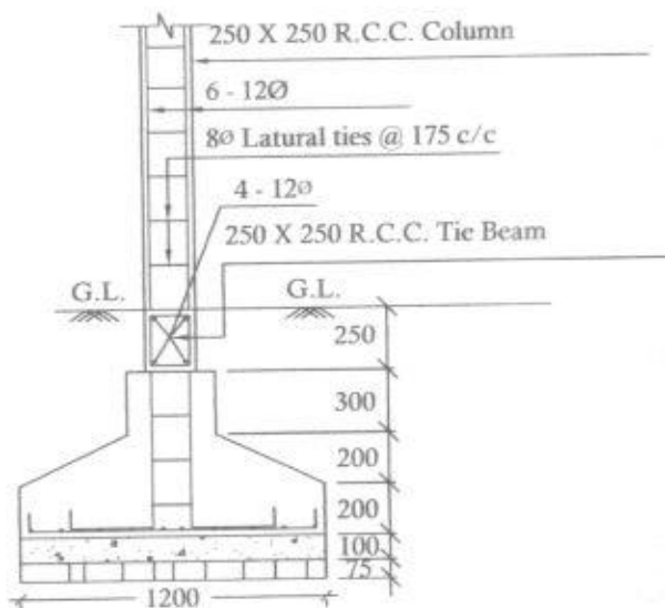
DETAILS OF R. C. C COLUMN
