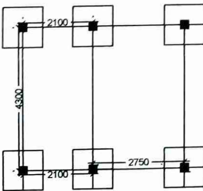
LAYOUT PLAN
